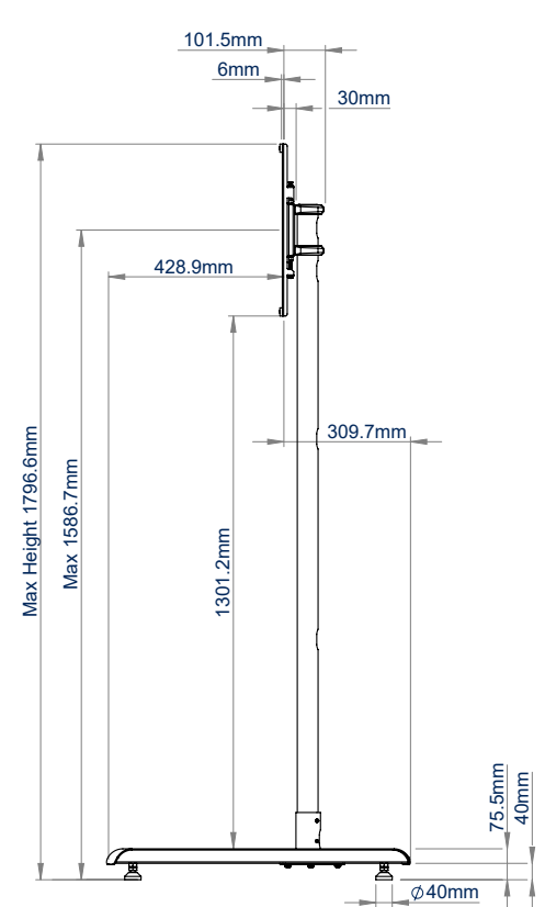
SIDE VIEW WITH LEVELLING FEET
