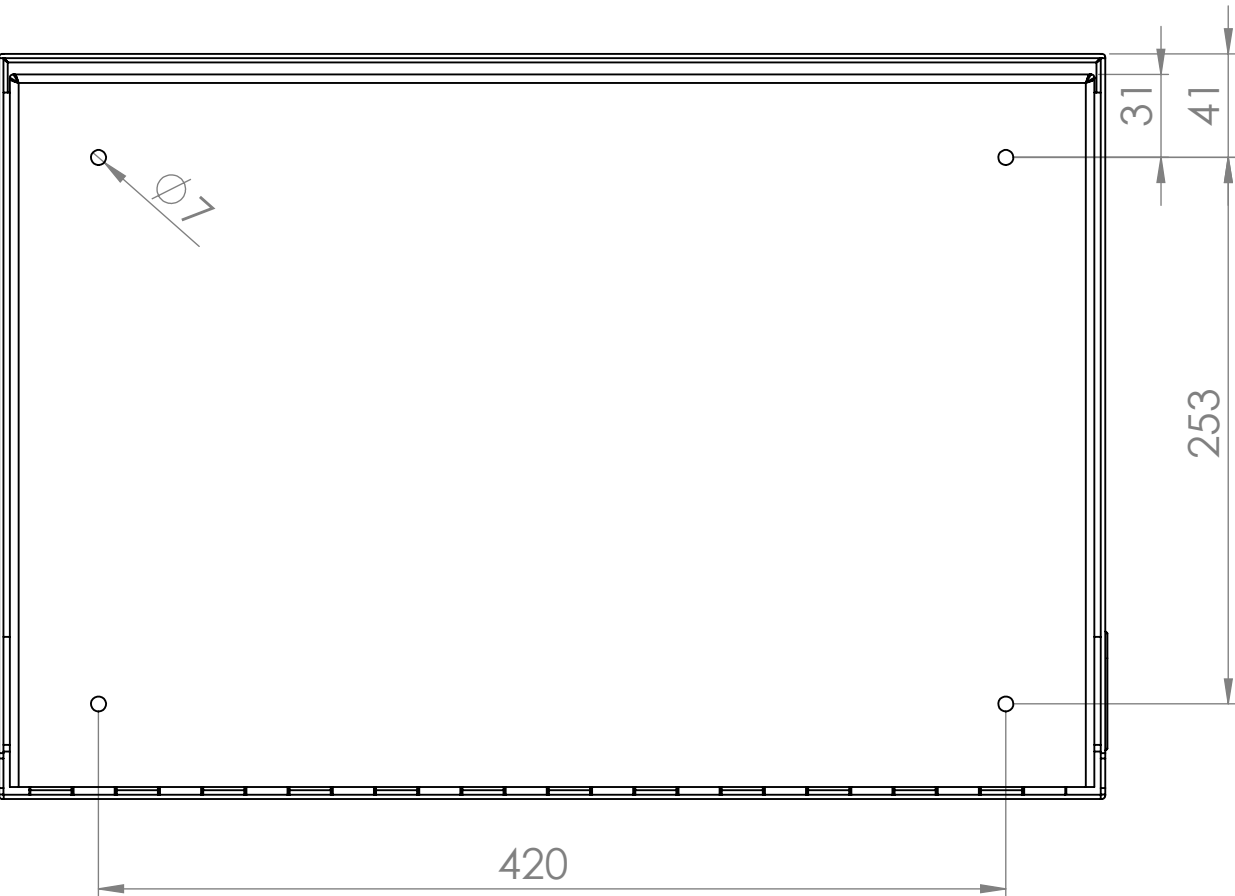
Rear - Mounting pattern
