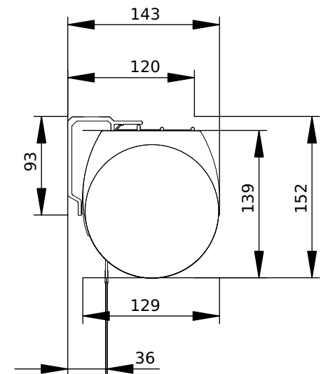
Case Side Detail
