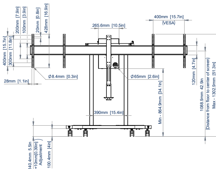
FRONT VIEW LOWEST POSITION
